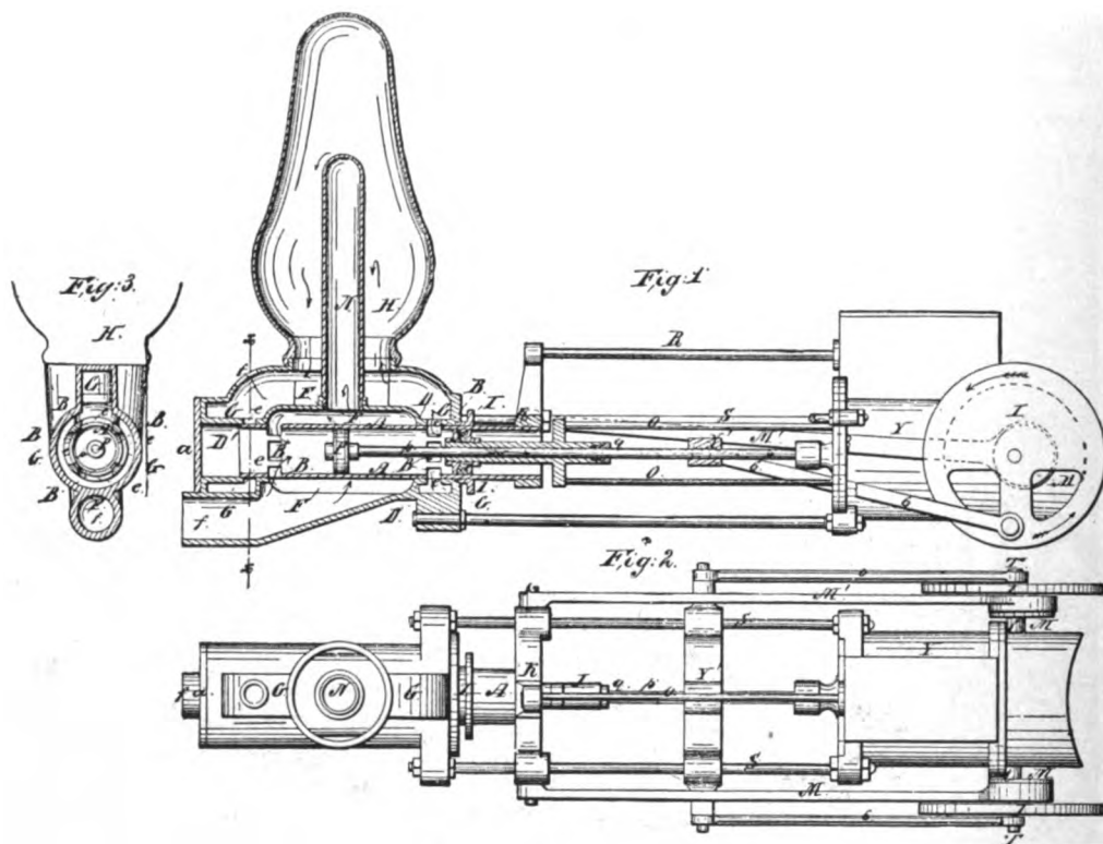
JOHNSON PUMP, PATENTED 1860.
