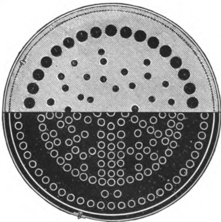
SECTION OF SILSBY BOILER.
