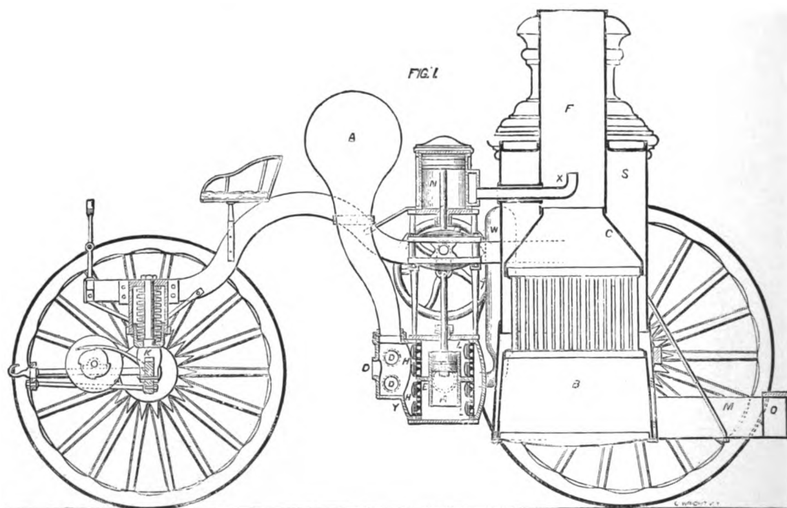
VERTICAL SECTION OF GOULD ENGINE.
