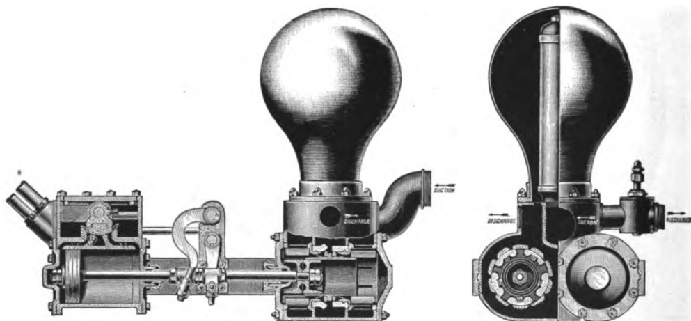
SECTIONS OF CLAPP & JONES VILLAGE ENGINE.
