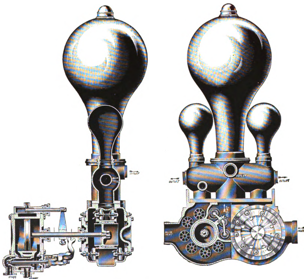
SECTION OF BUTTON ENGINE.
