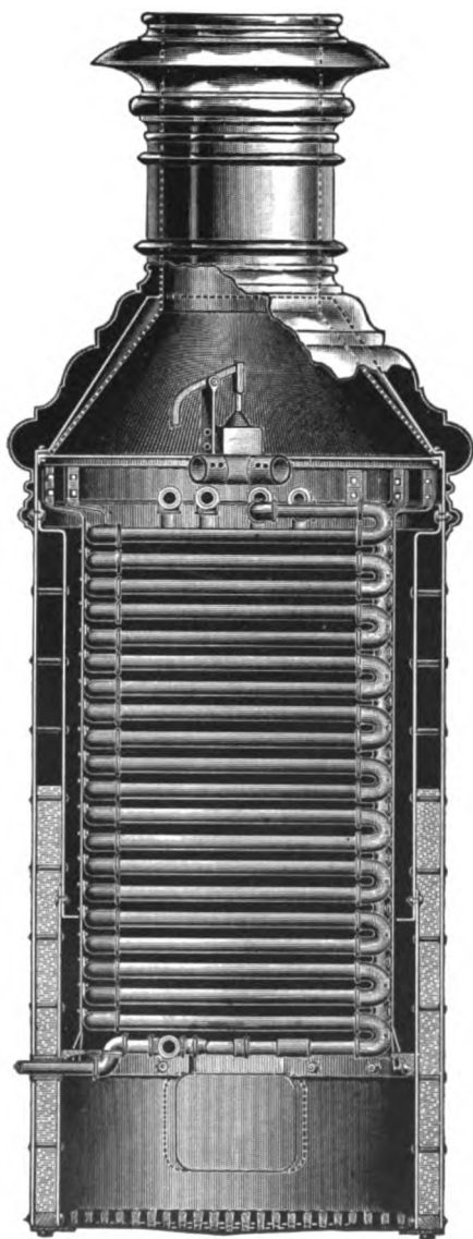
MODERN AHRENS BOILER.
