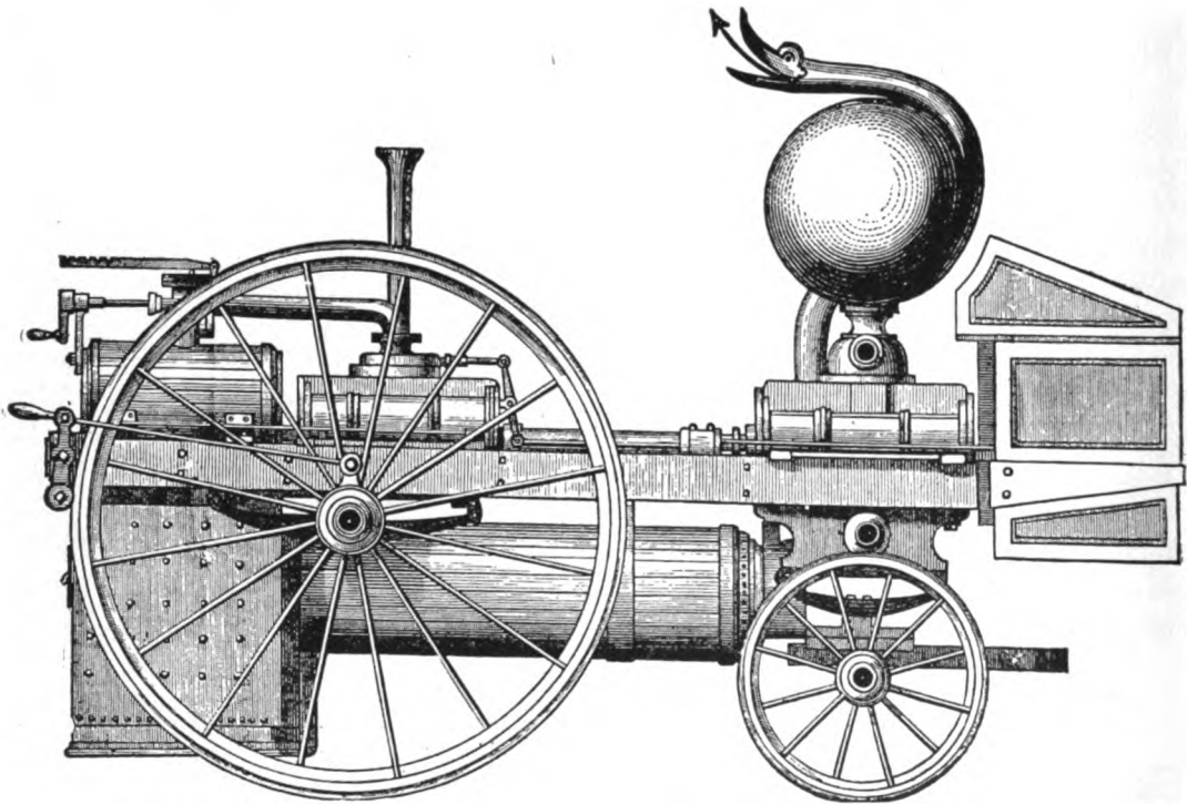
ERICSSON'S DESIGN FOR ENGINE.
