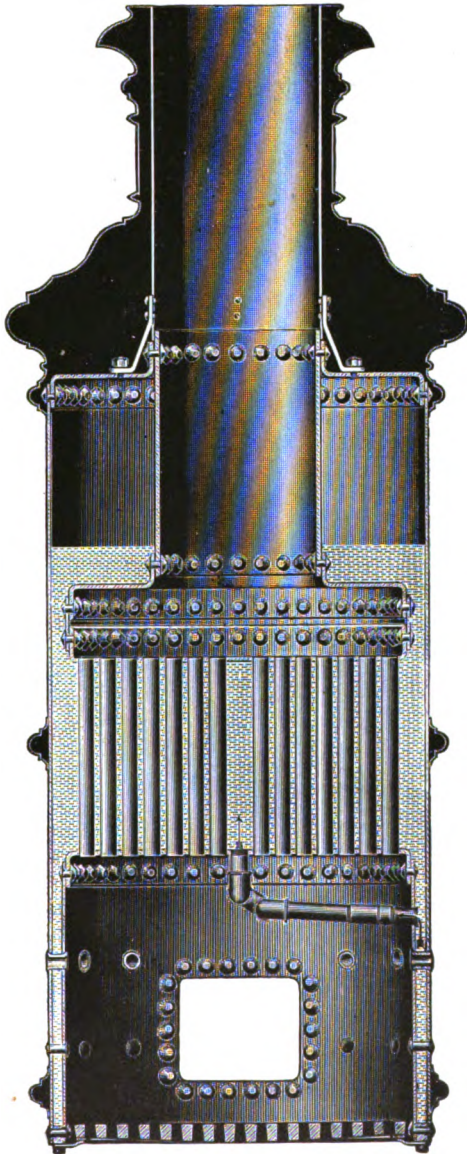
SUBMERGED FLUE BOILER.
