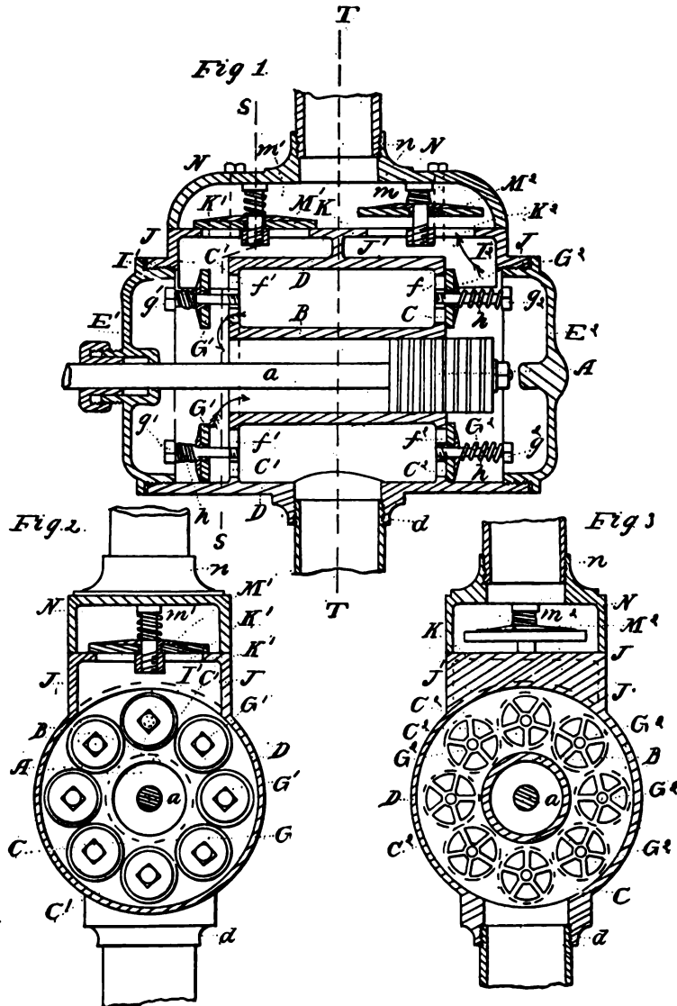
HORIZONTAL PUMP, PATENTED BY M. R. CLAPP, 1865.
