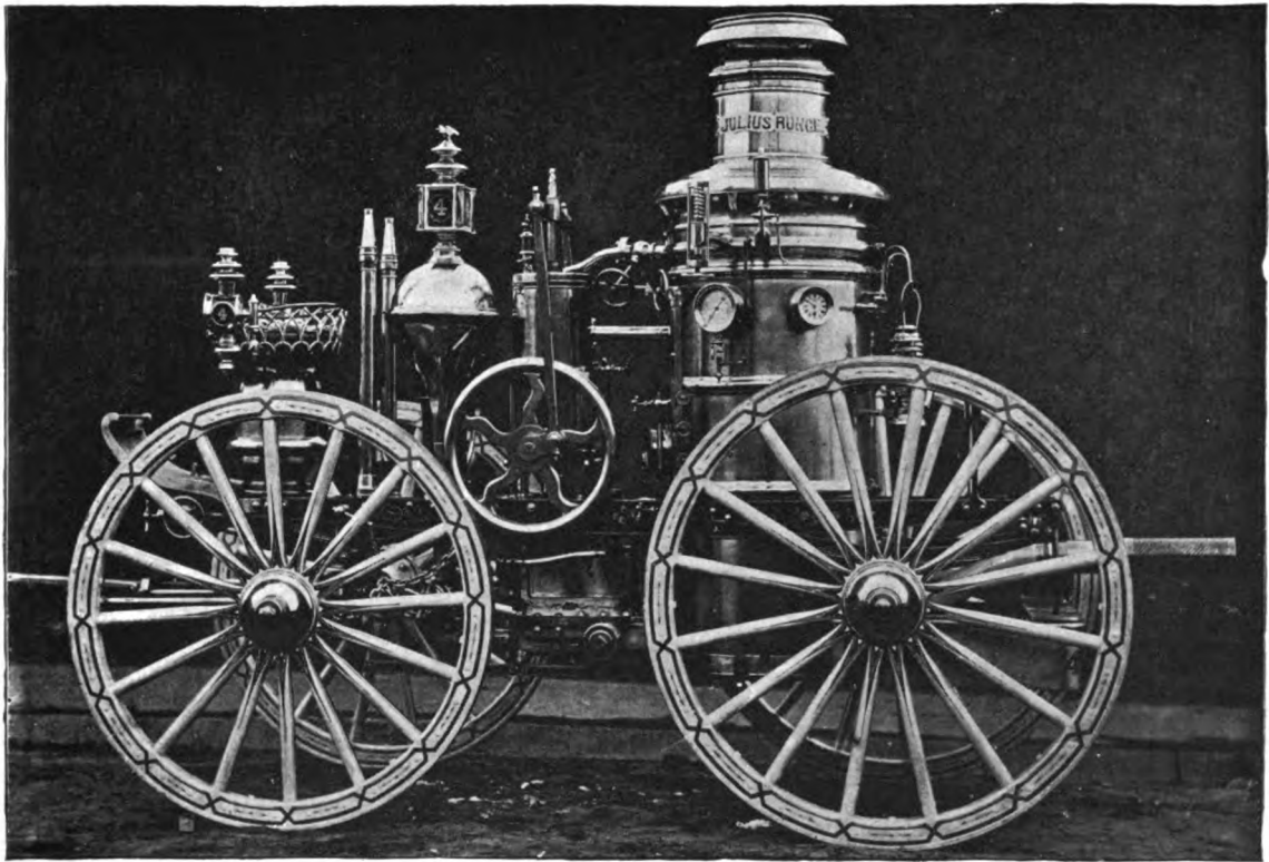
SINGLE ENGINE BUILT BY P. S. SKIDMORE.
