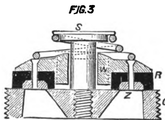
GOULD PUMP VALVE.
