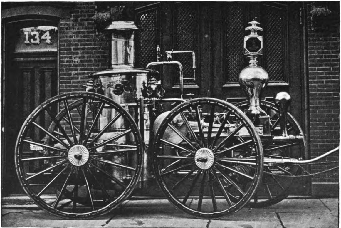
CONTINENTAL ENGINE NO. 9, BROOKLYN, N. Y. Built by James Smith.
