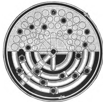
BOTTOM SECTION OF CLAPP & JONES BOILER.
