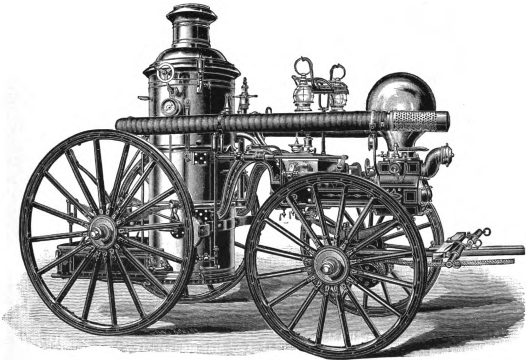
CLAPP &amp; JONES VILLAGE ENGINE.
