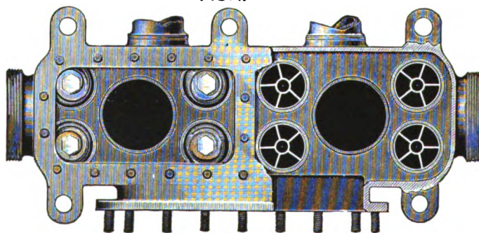
FIG. 3. SECTION OF "NEW AMERICAN" PUMP.
