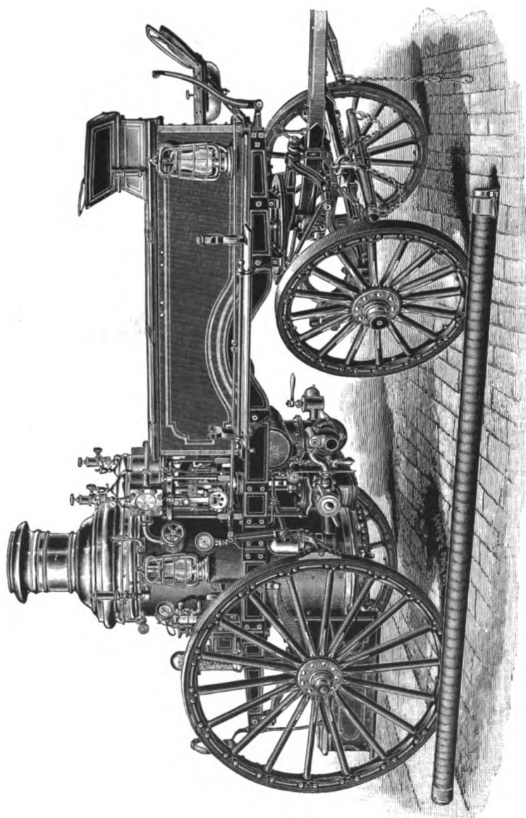
COLUMBIAN ENGINE.
