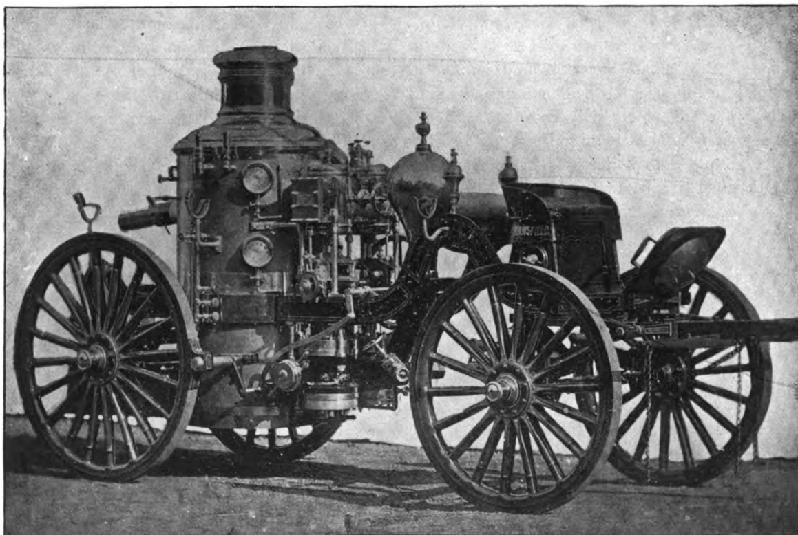
DOUBLE PISTON ENGINE.
