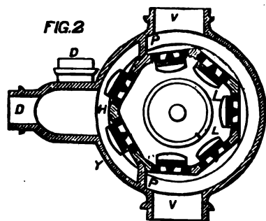
HORIZONTAL SECTION OF GOULD PUMP.
