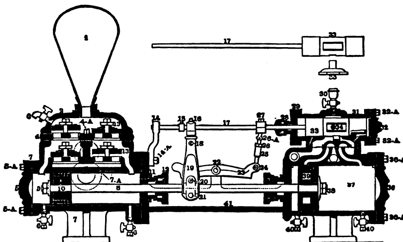
PARTS OF KNOWLES PUMP.
