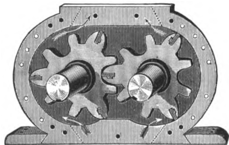
SILSBY ROTARY PUMP.
