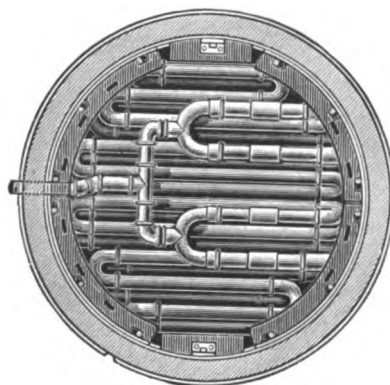
BOTTOM VIEW OF AHRENS BOILER.
