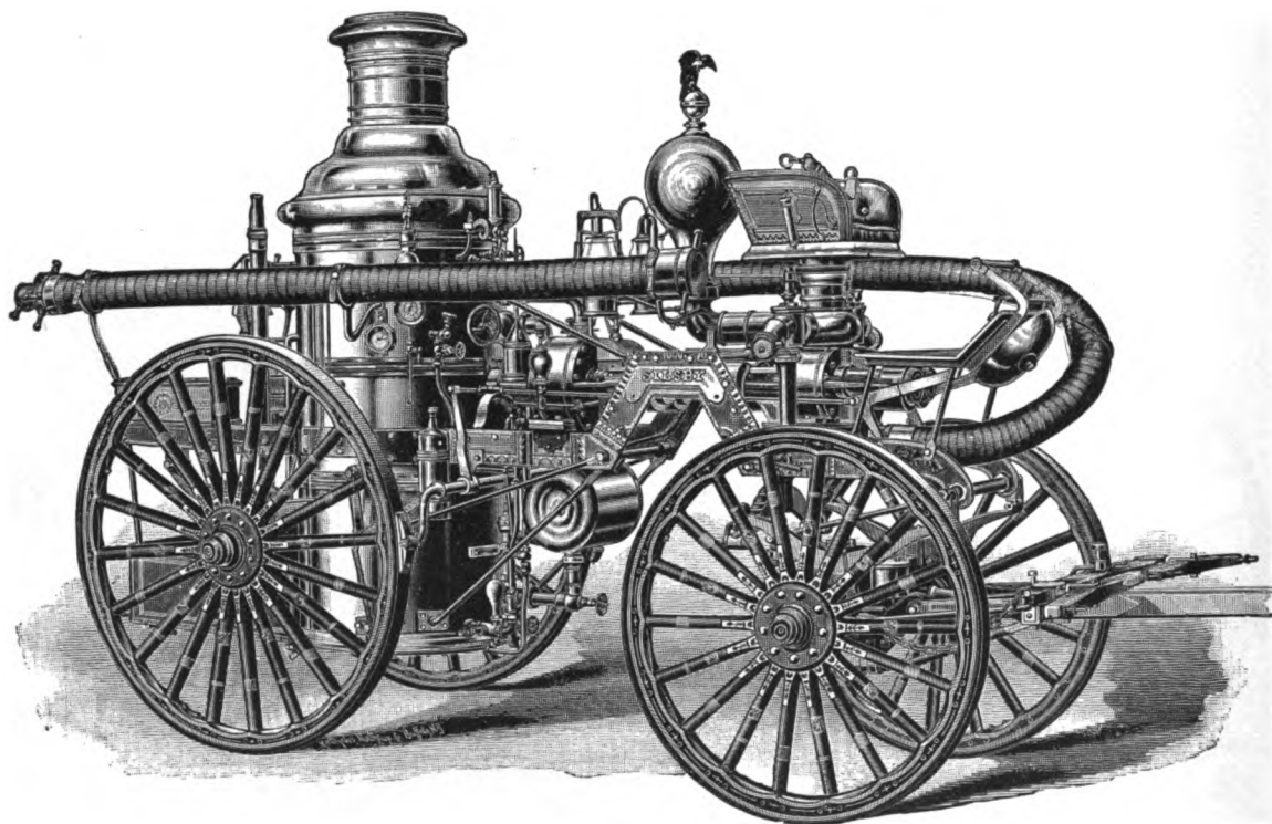
MODERN SILSBY ENGINE.
