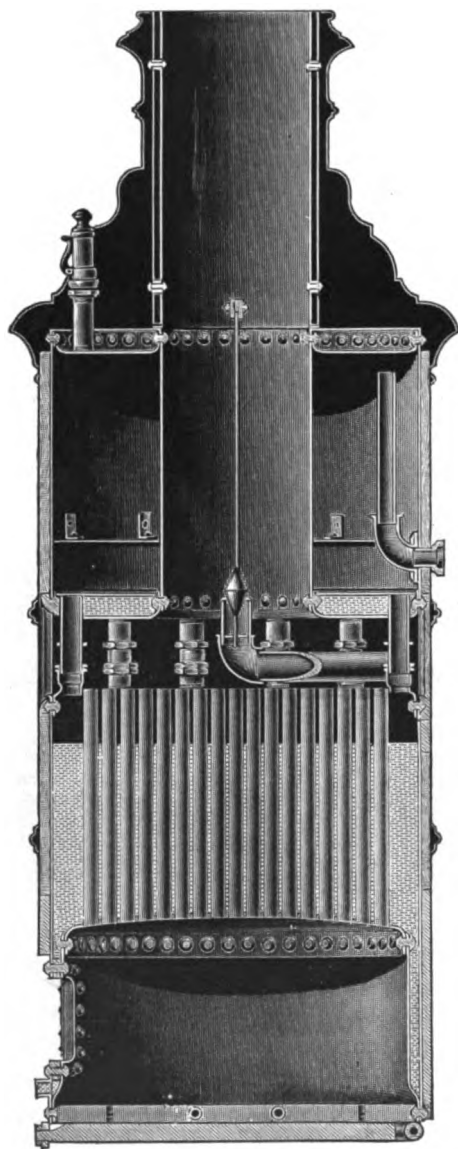
MODERN BUTTON BOILER.
