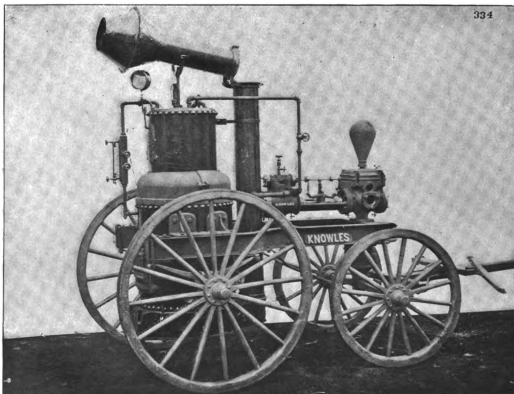
KNOWLES STEAM ENGINE.
