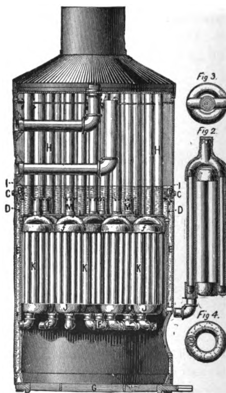
LA FRANCE NEST-TUBE BOILER.
