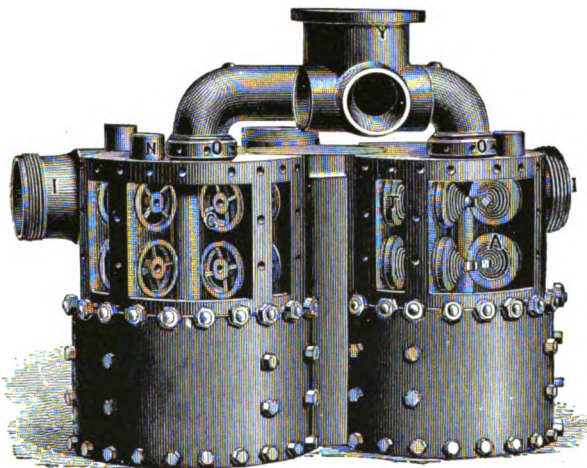
LA FRANCE PUMP.
