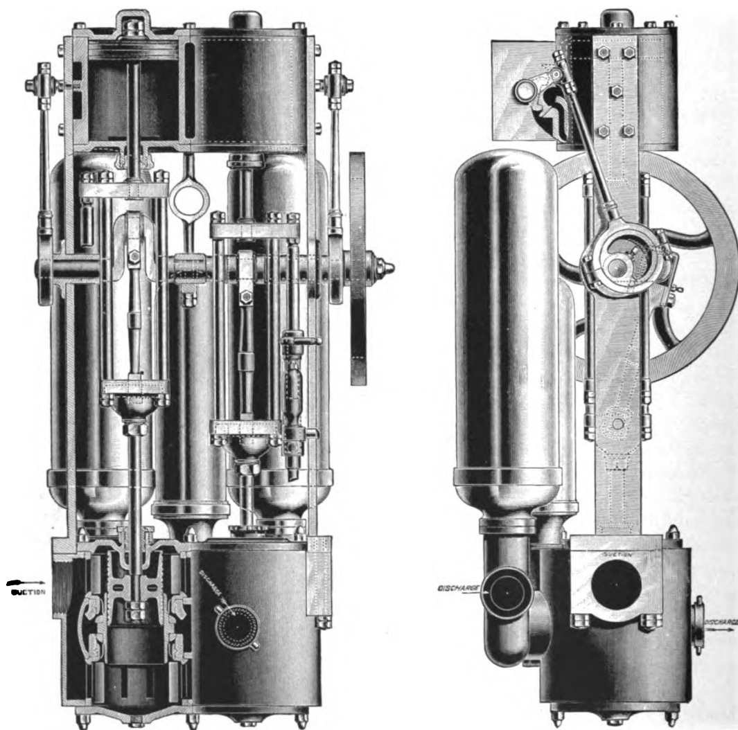
SECTION OF CLAPP &amp; JONES DOUBLE VERTICAL ENGINE.
