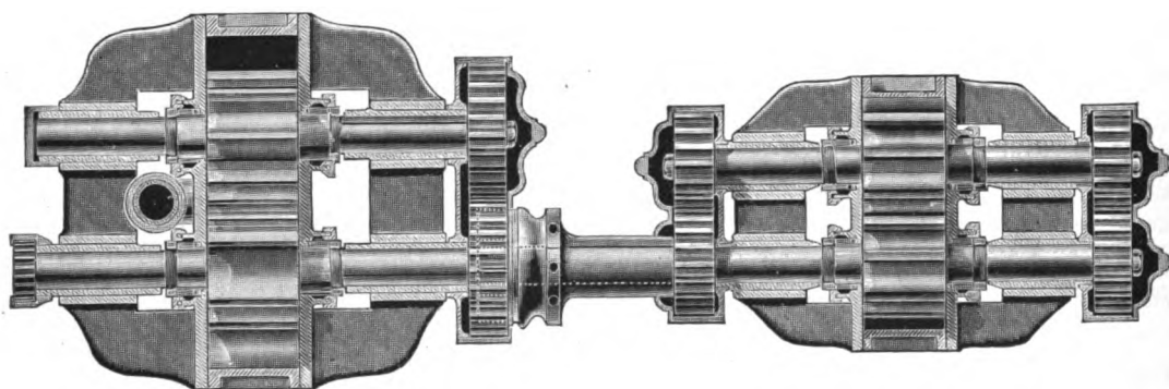
SECTION OF SILSBY PUMP AND STEAM CYLINDER.
