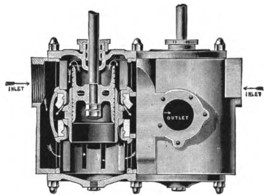
SECTION OF CLAPP & JONES PUMP.
