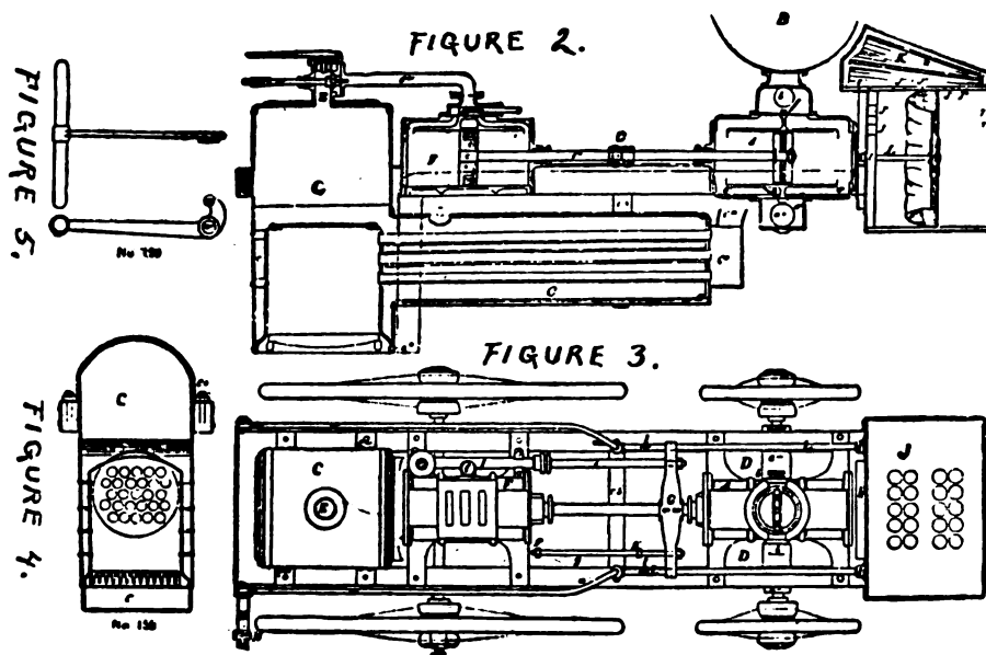
SECTIONAL VIEW OF ERICSSON'S ENGINE.
