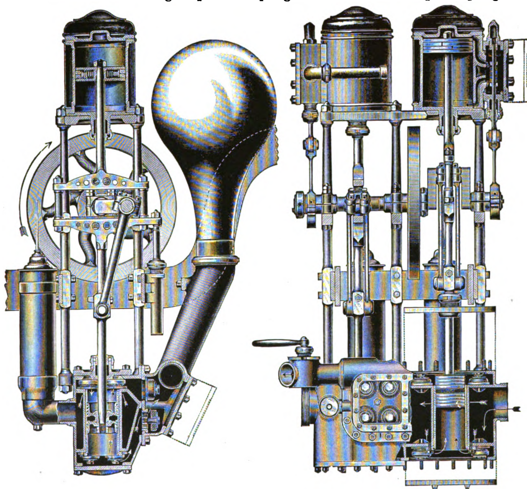
SECTION OF "NEW AMERICAN" ENGINE.
