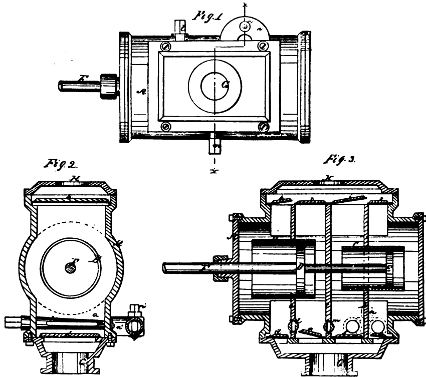
HORIZONTAL PUMP PATENTED BY J. N. DENNISSON, 1866.
