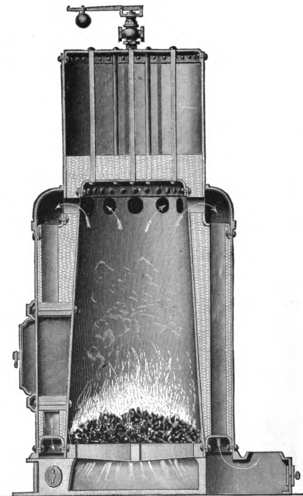
SHAPLEY PATENT BOILER.
